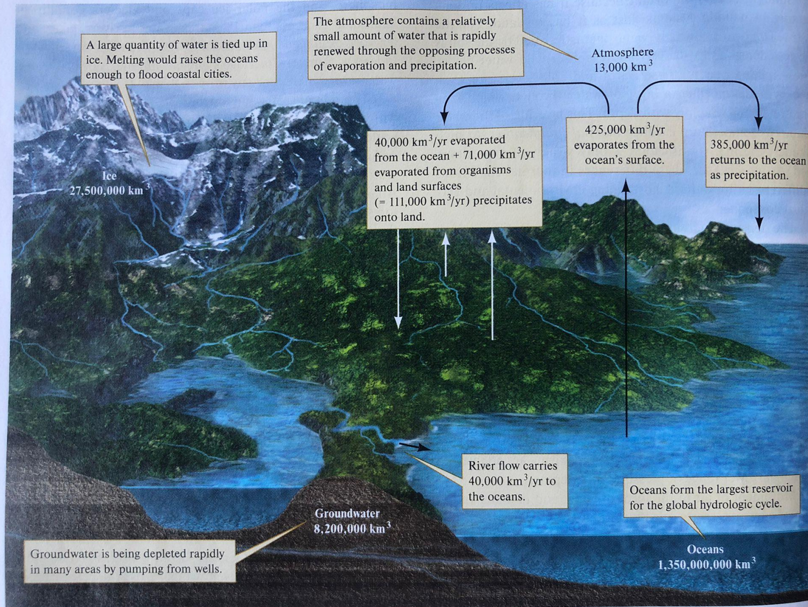
Figure 3.2 The hydrologic cycle (data from Schlesinger 1991).
