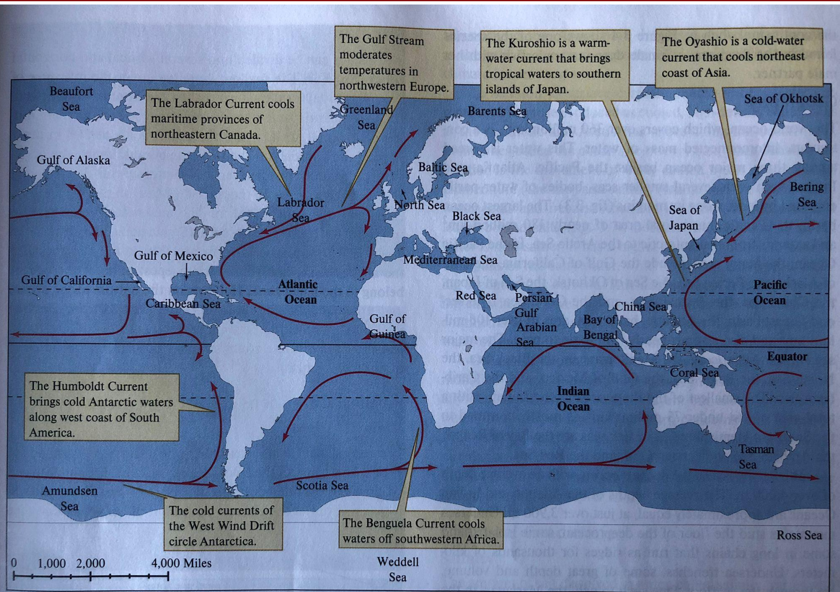
Figure 3.3 Oceanic circulation, which is driven mainly by the prevailing winds under the influence of the Coriolis effect, moderates earth's climate.
